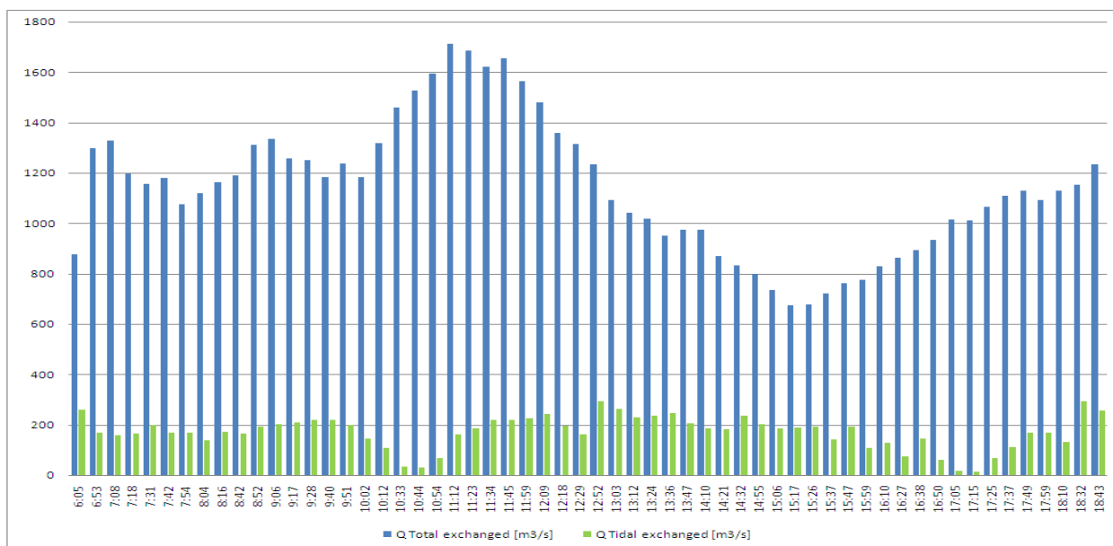
Figure 5-10 Total exchanged discharge versus exchanged discharge due to tidal filling at DGD on 24/09/2008
