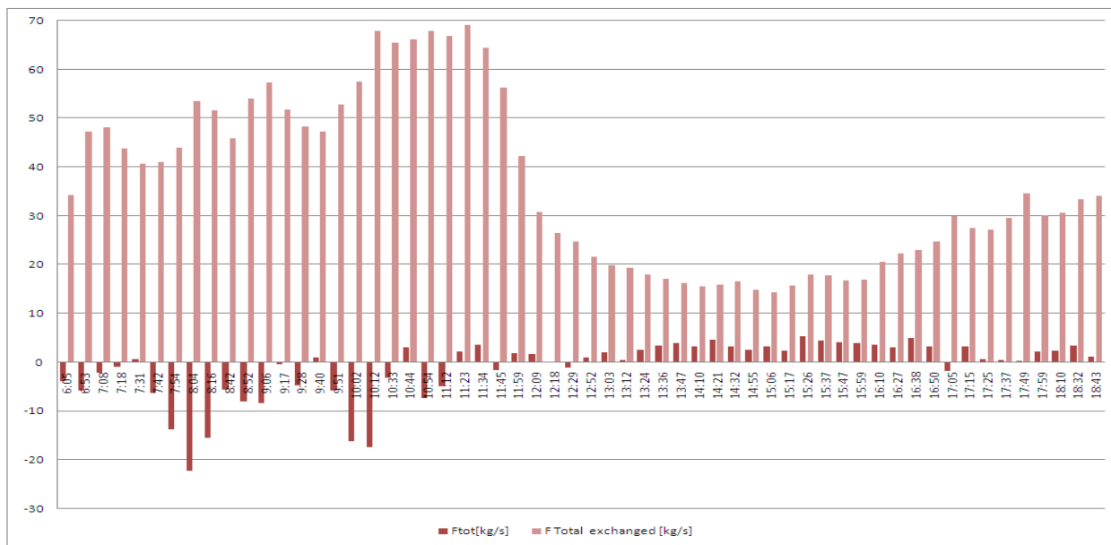
Figure 5-14 Total sediment flux versus total sediment exchange at DGD on 24/9/2008 (negative values represent incoming sediment)
