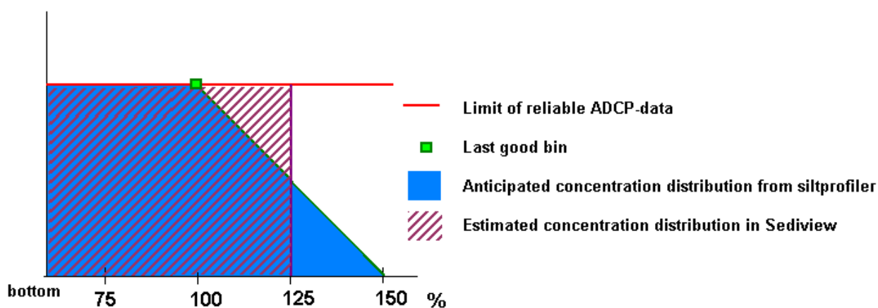
Figure 4-3: Principal of bottom estimate of the sediment concentration
