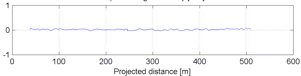
Depth Averaged Velocity [m/s]
