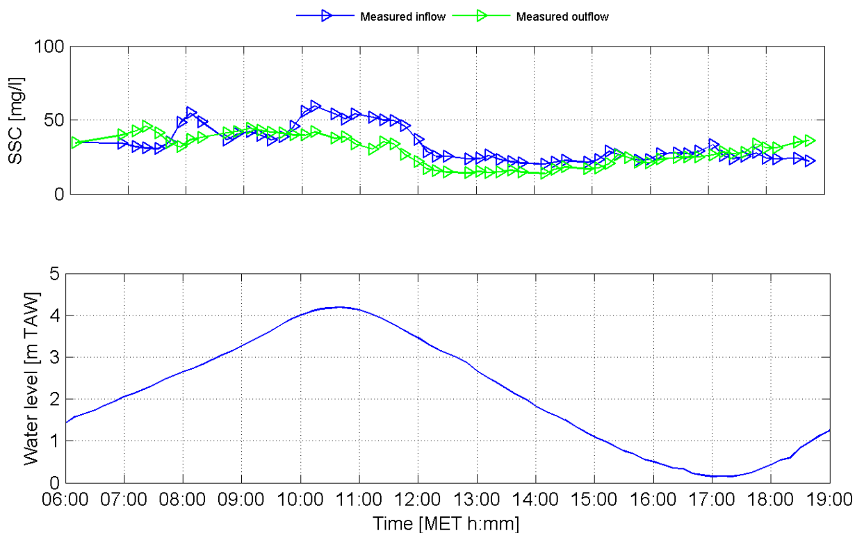
Figure 5-1 Average incoming and outgoing SSC over a complete tidal cycle on 24/9/2008
