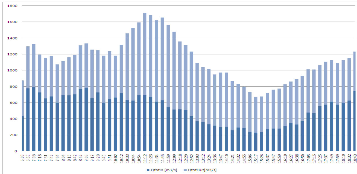
Figure 5-9 Total incoming and outgoing discharge at DGD on 24/09/2008
