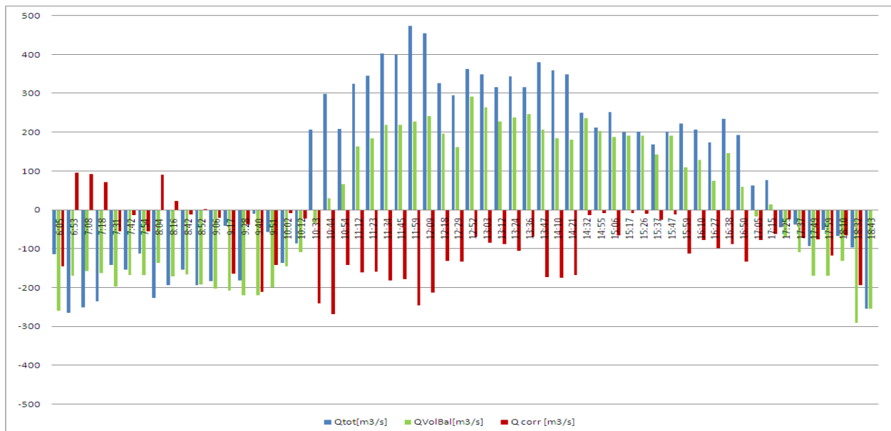
Figure 5-11 Measured residual discharge (Qtot) versus theoretical residual discharge (QVolBal) and correction offset (Qcorr) at DGD on 24/09/2008 (negative values represent incoming water)
