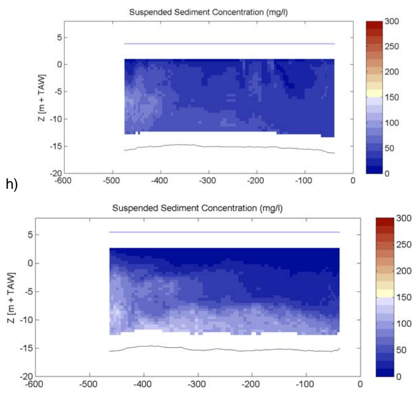
Figure 5-8: a) Suspended sediment concentration on 17/11/2005, b) on 22/03/2006, c) on 27/09/2006, d) on 24/10/2007, e) on 11/03/2008, f) on 19/06/2008, g) on 26/06/2008, on h) 24/09/2008 & i) on 30/09/2008 at 1h after high water
