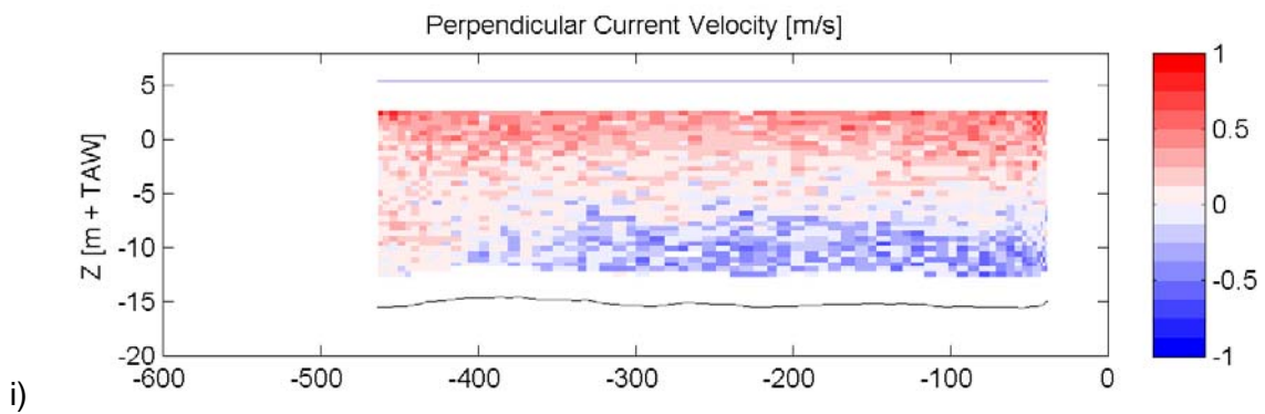
Figure 5-7: a) Perpendicular current velocity on 17/11/2005, b) on 22/03/2006 , c) on 27/09/2006, d) on 24/10/2007, e) on 11/03/2008, f) on 19/06/2008, g) on 26/06/2008, on h) 24/09/2008 and i) 30/09/2008 at 1h after high water
