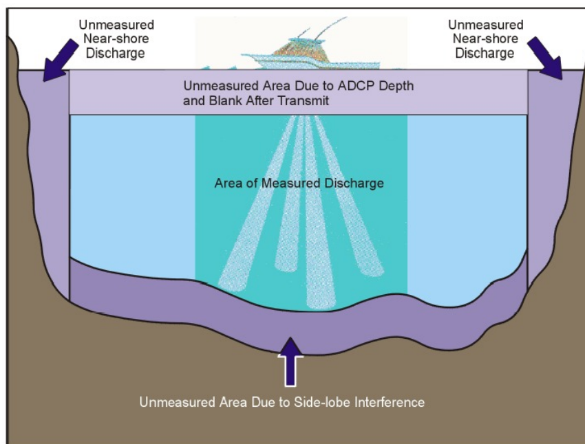
Figure 4-1: Unmeasured regions in the cross section (from RD Instruments, 2003)
