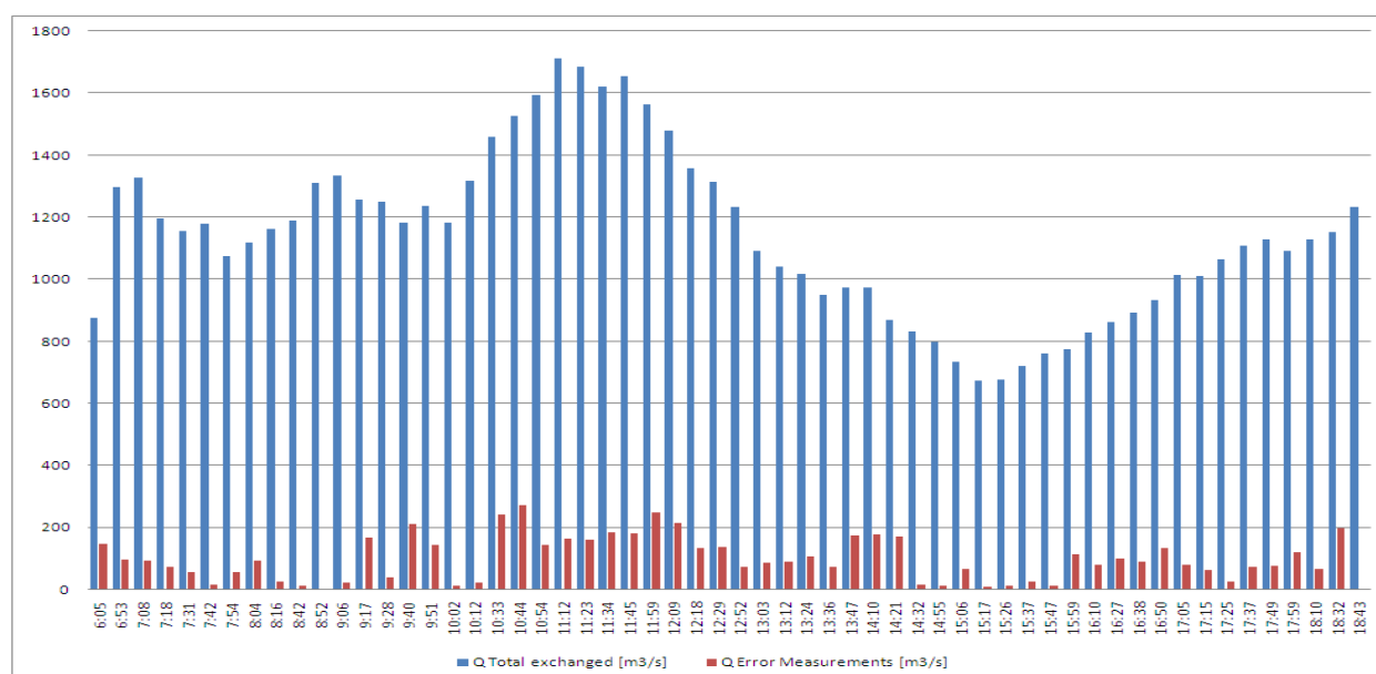
Figure 5-12 Absolute error in total water exchange versus total water exchange at DGD on 24/09/2008
