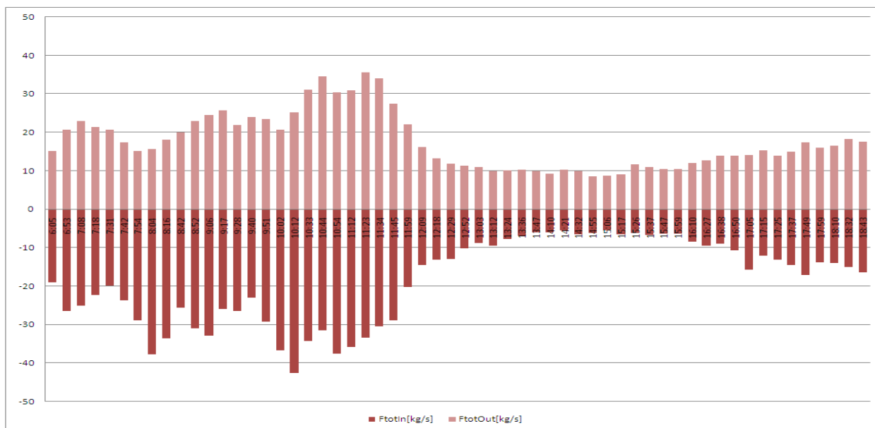
Figure 5-13 Total incoming and outgoing sediment flux at DGD on 24/09/2008 (negative values represent incoming sediment)
