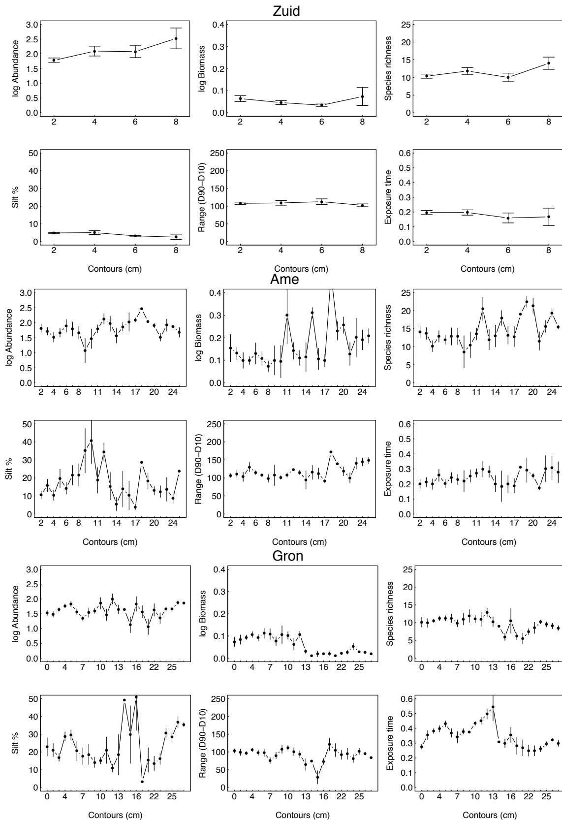
Figure 4. Trends in abundance ( \log_{10} ), biomass ( \log_{10} ), point richness, silt (<63%), range in sediment grain sizes (D 90 -D 10 ) and the fraction of exposure time with respect to the predicted contour intervals of subsidence in the Ameland (Ame) and Groningen (Gron) gas extraction areas.
