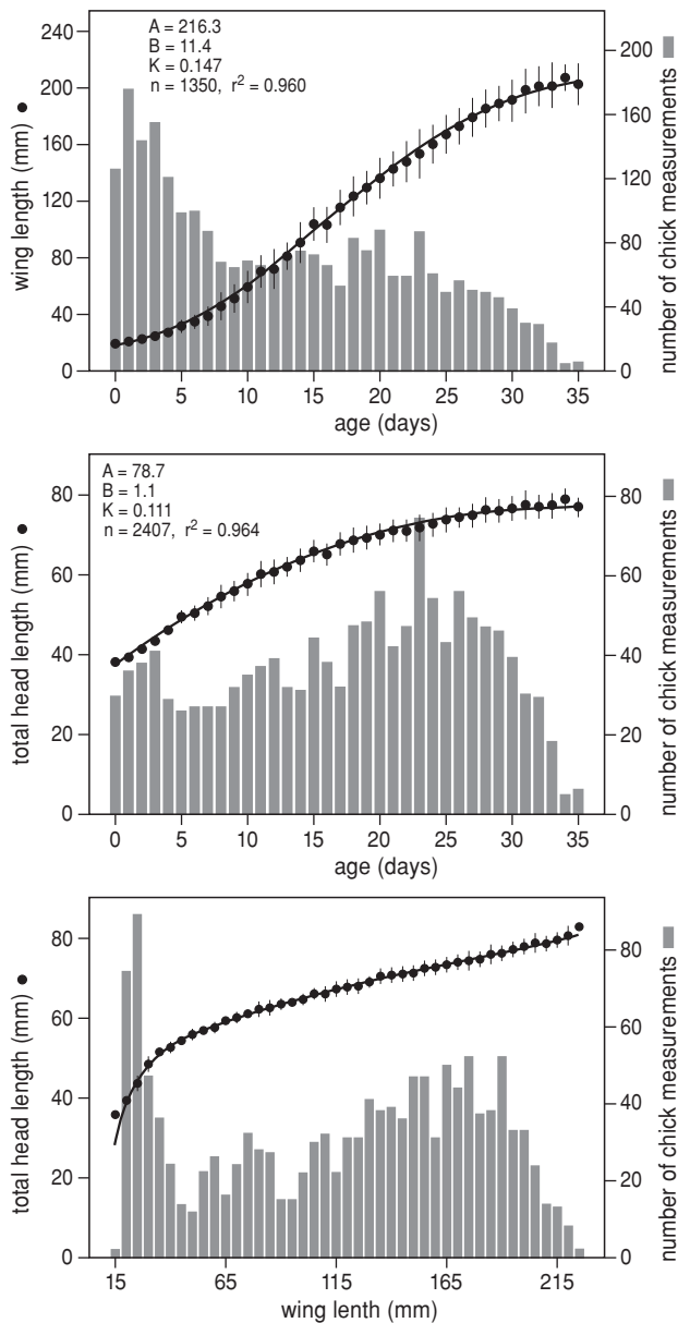
Figure 6.1. Development of wing and total head length (dots \pm sd) with the age of enclosed Sandwich Terns on Griend in 1992-1998 (upper and middle graphs). Drawn lines are logistic growth curves (length = A / (1 + B * e^{-K*age}) ) for which the parameters are shown in the top of the graphs. The lower graph shows the relationship between wing length (15 = 12.5 - 17.4 mm, 20 = 17.5 - 22.4 mm, etc.) and total head length. The drawn line is a quadratic by linear curve: total head length = 57.1 + 69.5/(1-0.22*wing\ length) + 0.11*wing\ length , n = 1350 , r^2 = 0.978 ). Bars denote the number of chick measurements (right axis).
