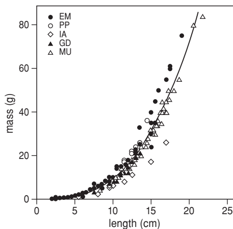
Figure 8.3. The relationship between mass (g) and total length (cm) of roundfish, caught on different places in the Archipelago dos Bijagós from October to December 1992 by beam trawls by H. Witte. \text{Mass (g)} = 0.01167 * \text{Length (cm)}^{2.915} , r^2 = 0.94 , n = 184 ; EM = Eucinostomus melanopterus , GD = Galeiodes decadactylus , IA = Ilisha africana , MU = mullet ( Liza grandisquamis , L. ramada , Mugil cephalus or M. curema ) and PP = Pomadasyd peroteti .
