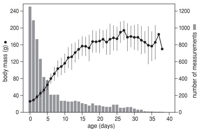
Figure 5.1. Increase in body mass ( \bar{X} \pm SD ) of tern chicks in 1995-1996.
