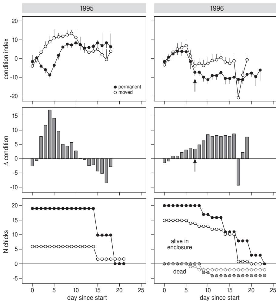
Figure 5.5. (upper graphs) Variation in chick condition ( \bar{X} \pm \text{SD} ) for the permanent and moved enclosures throughout the experiment in 1995 and 1996. (middle graphs) Difference in average condition index between the two enclosure types. Positive values indicate that the chicks in the moved enclosure were in better condition than those in the permanent enclosure. The arrow indicates when the enclosure was moved 25 m further away. (lower graphs) Number of chicks alive in the enclosure and number of chicks found dead.
