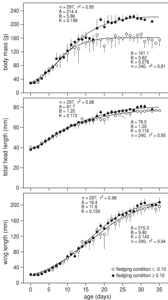
Figure 6.3. Pre-fledging development (means \pm sd) of body mass (upper graph), total head length (middle graph) and wing length (lower graph) in Sandwich Tern chicks fledging in poor (fledging condition \leq -0.10 ) and good condition (fledging condition \geq 0.10 ). Only chicks that reached an age of 25 days were included in the analysis. Drawn lines represent logistic growth curves for which the parameters are shown in the top of the graph.
