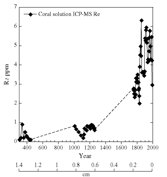
Figure 5. Trace metal analysis for rhenium (Re) concentration was performed on discrete growth layers using solution ICP-MS. In the outer, mid, and center regions of the radial transect, samples were taken at intervals of approximately 39, 97, and 143 \mu\text{m} , respectively. Rhenium concentrations were elevated in the outermost region of the sample (GOM-JSL09-3728-BC1), consistent with the laser results (Figure 4).
