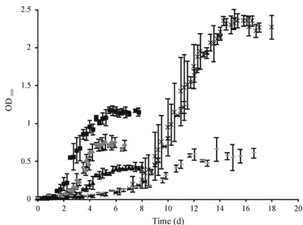
Fig. 3. Growth on 1% methanol (v/v) for different Methyloceanibacter spp over time. R-67174 (▲), R-67175 (X), R-67176 (◆), R-67177 (-), Gela4T (■). All strains were grown till stationary phase (based on at least 3 replicate measurements) and demonstrated clear differences in lag phase, growth rate and maximum cell density (see Table 1).
