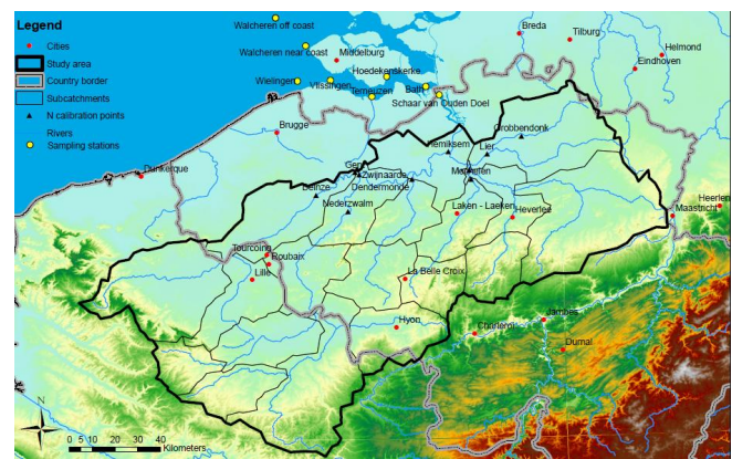
Fig. 2. Scheldt catchment and its tributaries, as well as the locations of stations used for verification (Figs. 3 and 4). The station Hemiksem forms the transition from river to estuary.
