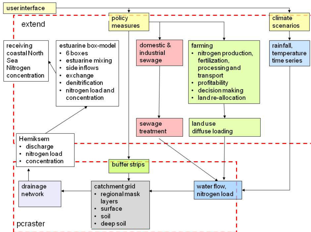
Fig. 1. General structure of the model suite of water and nitrogen flowing through the Scheldt catchment, developed using PCRaster and ExtendSim. Policy measures and climate scenarios can be manipulated by the user.
