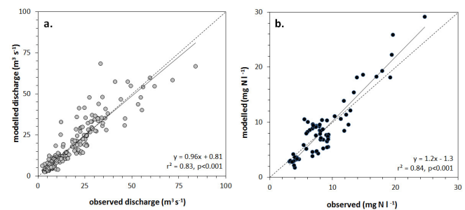
Fig. 4. Performance of the calibrated ExtendSim estuarine box model for the estuarine boxes along the Westerschelde after 1 yr of model run (2006). The intercept did not differ significantly from zero ( p = 0.21 ) and the slope is not significantly different from one ( p = 0.12 ).
