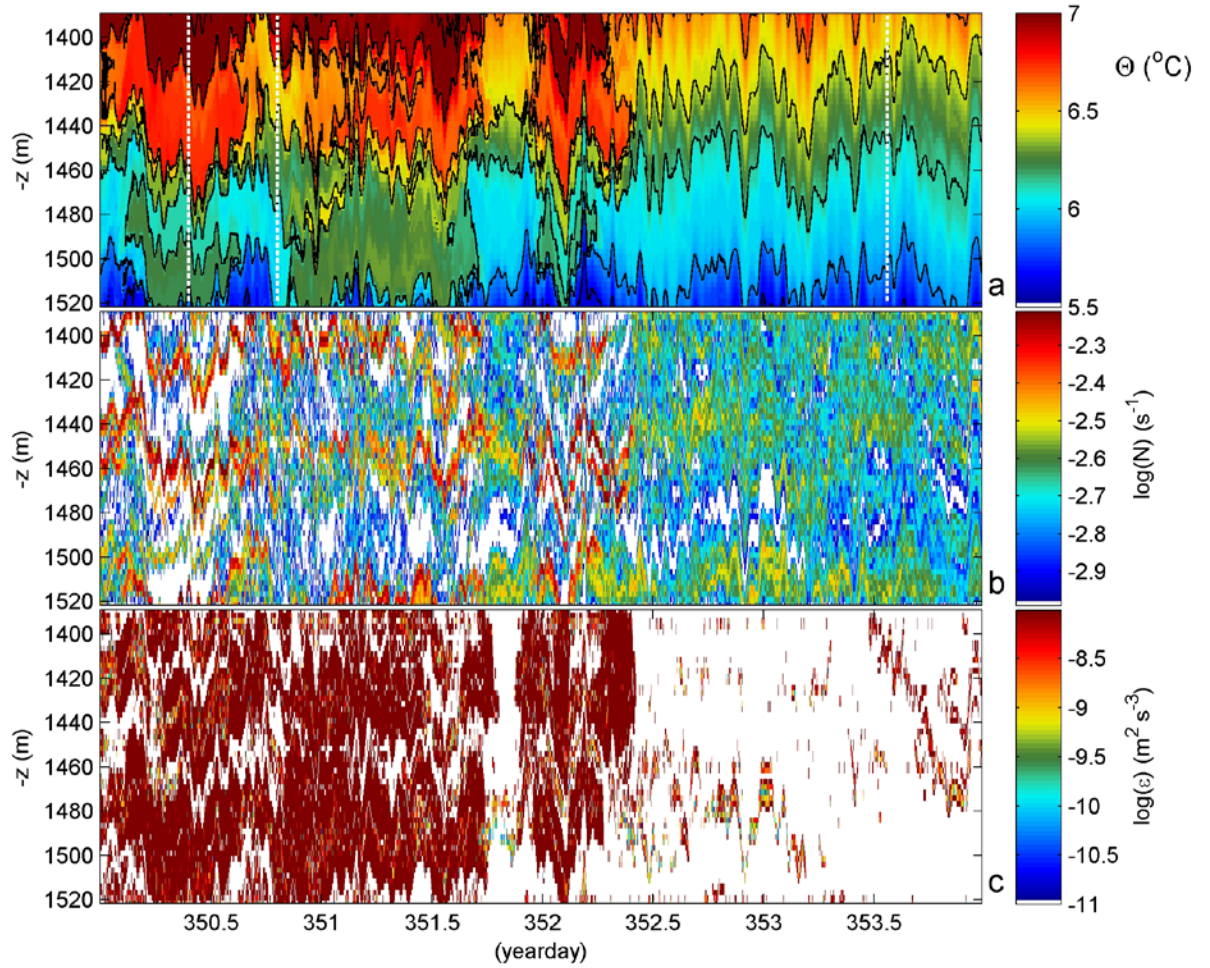
Figure 5. Four day time-depth series of T-sensor data around the transition between intrusion-dominated step-like stratification up to day 352.5 and more gradual stratification after day 352.5 assumed to be related with the passage of a Meddy. (a) Conservative Temperature with black contours drawn at 0.25^{\circ}\text{C} increments and the vertical white-dashed lines indicating the times of profiles of Fig. 6. (b) As in Fig. 4b. (c) As in Fig. 4c.
