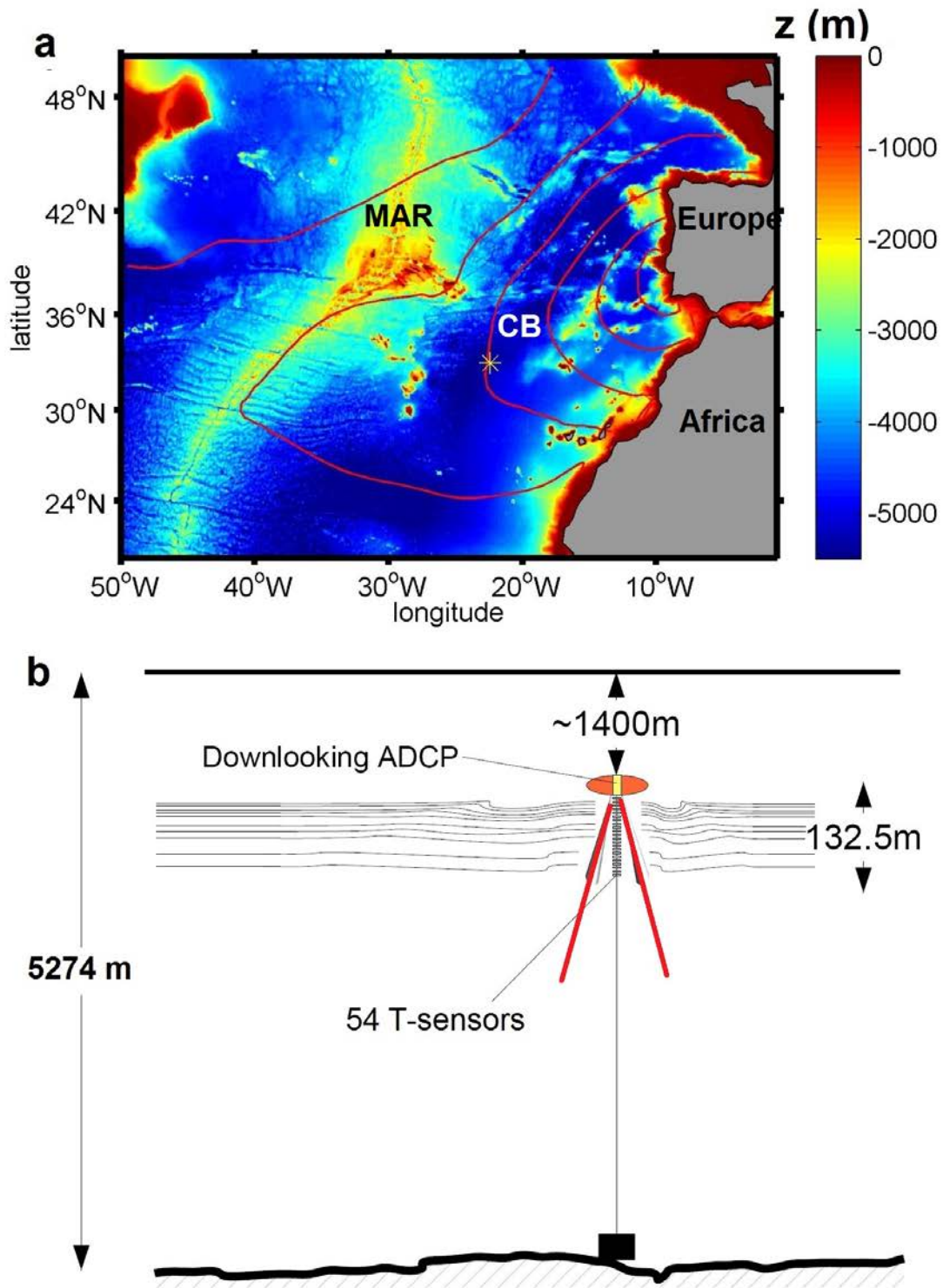
Figure 1. Mooring. (a) Site (asterisk) in the Canary Basin ‘CB’ of the NE-Atlantic, with annual mean salinity contours at 1400 m from World Ocean Atlas 2005 (Antonov et al., 2006). MAR denotes Mid-Atlantic Ridge. Individual Meddies have approximately the horizontal size of the asterisk. (b) Configuration.
