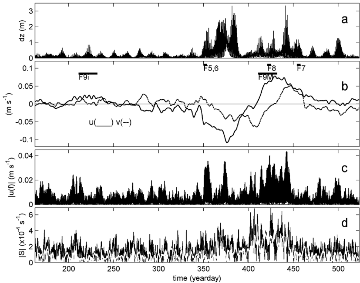
Figure 2. Current velocities and mooring motion, for the first year of data. (a) Vertical top-buoy displacement due to current drag as estimated from tilt and pressure information. (b) Horizontal current components averaged over the range between 1400 and 1530 m and low-pass filtered using a phase-preserving double-elliptic filter with ripple suppression and cut-off at 0.2 cpd. Solid graph is u - (positive Eastward), dashed graph v - (positive Northward) component. The periods of Figs 5-6, 7, 8 and 9 are indicated with 'F' and number. (c) Magnitude of band-pass filtered near-inertial u -component. (d) Shear-magnitude over the 132 m range of T-sensors from filtered ADCP-data. A near-inertial band-pass filter yields the solid graph and a 0.2 cpd cut-off low-pass filter the white graph.
