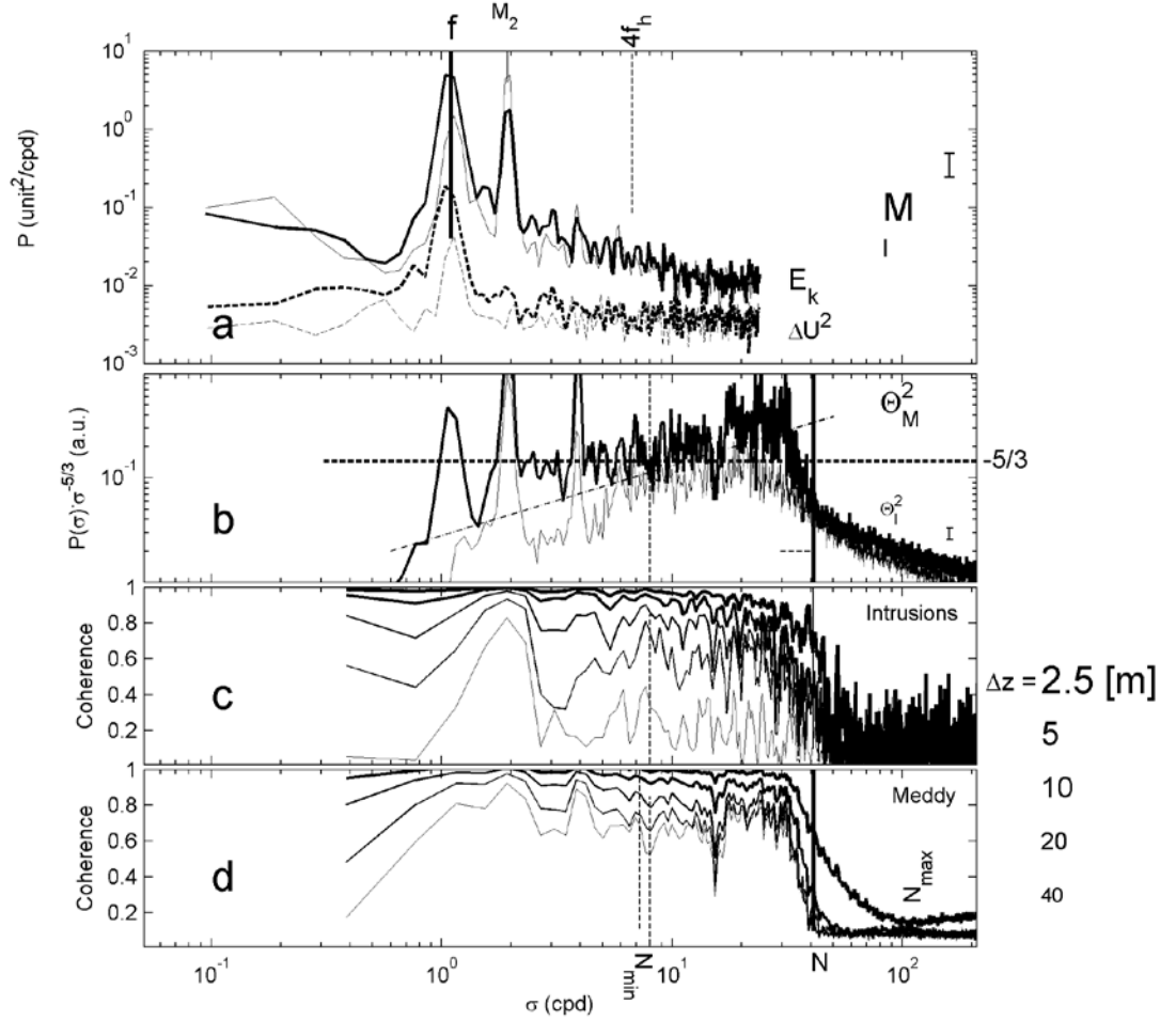
Figure 9. Spectral overview for the periods between days 211 and 232, representing a period dominated by intrusions ‘I’ (thin graphs in a., b.), and between days 411 and 432, representing a Meddy ‘M’ passage above (bold graphs in a., b.). (a) Moderately smoothed (30 degrees of freedom, dof) spectra of kinetic energy from ADCP averaged over vertical bins 1-14 (solid), which corresponds with the range of T-sensors, and current velocity difference (between the depths of lower and upper T-sensor; dashed). The local inertial frequency f is indicated together with the semidiurnal tidal frequency M_2 and the local minimum buoyancy frequency N_{\min} \approx 4f_h , f_h denoting the horizontal Coriolis parameter. (b) Strongly smoothed ( \sim 100 dof) spectra of 20-s sub-sampled T-data representing M- and I-periods. Spectra are scaled with the inertial subrange slope of \sigma^{-5/3} , which is a flat horizontal line as in the dashes for reference. The dash-dot line slopes as +2/3 in this frame, representing a net spectral decay sloping like \sigma^{-1} . The vertical dashed line indicates N_{\min} and the solid vertical line the mean buoyancy frequency N during M-period, which may have a frequency extent as indicated by the thin horizontal dashed line during the I-period. (c) Coherence spectra for the I-period for all T-sensor-pairs at the separation distances indicated to the right (larger symbol = thicker line). (d) As c., but for the M-period.
