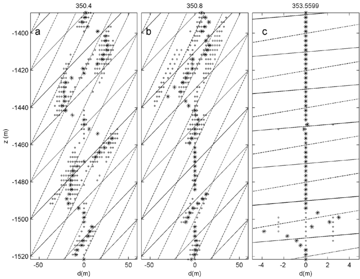
Figure 6. Three examples of ten consecutive profiles of displacements d (o) and their mean values at given depths (*) for times indicated above and along the vertical white-dashed lines in Fig. 5a. The grid consists of two slopes in the d - z plane: z/d = 1/2 (solid lines) and z/d = 1 (dashed lines). For the method see Section 2.3 and further in van Haren and Gostiaux (2014).
