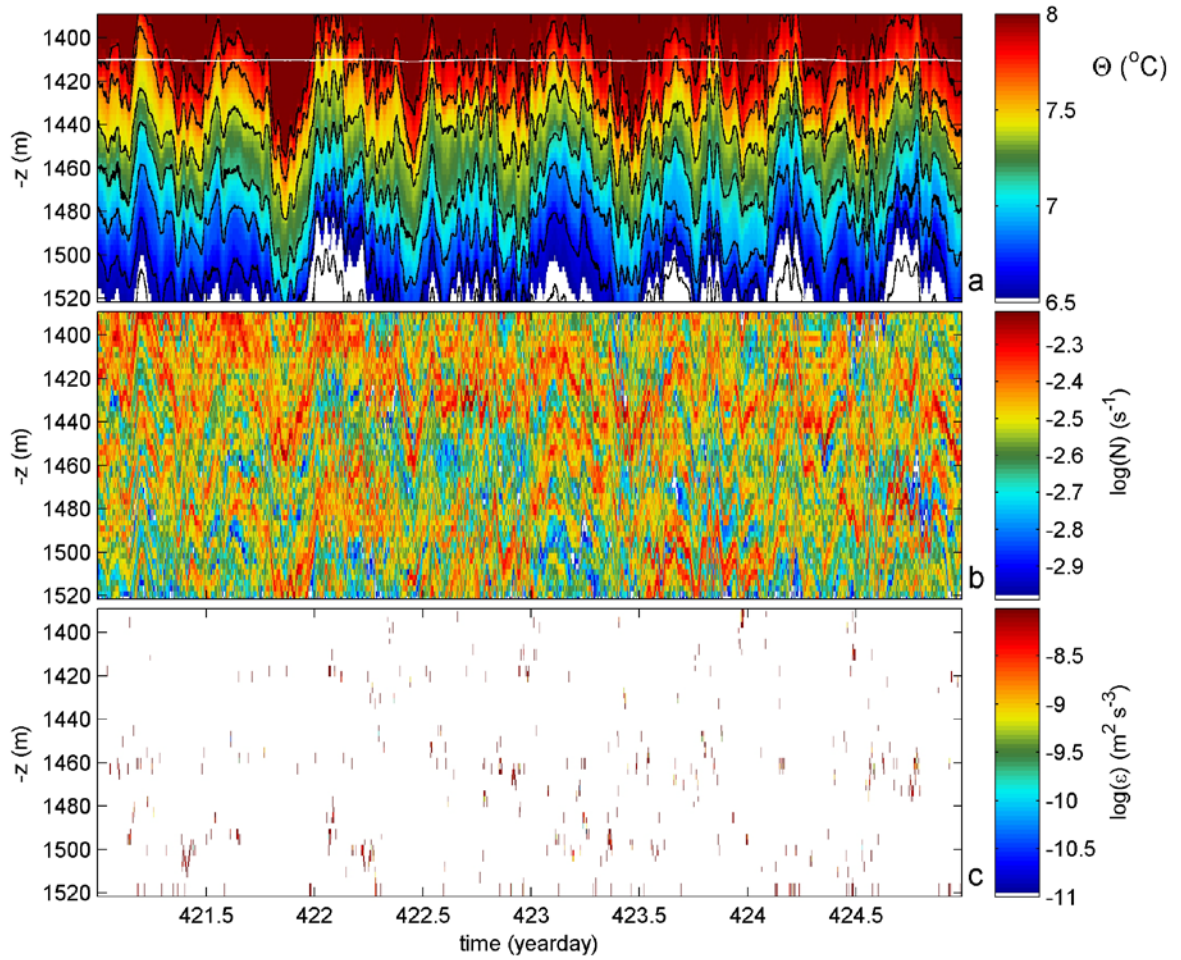
Figure 8. Same as Fig. 5, but during the passage of a Meddy. Note the different temperature range in a. The thin white line around -1410 m represents the time-series of the top-buoy vertical displacements of Fig. 2a.
