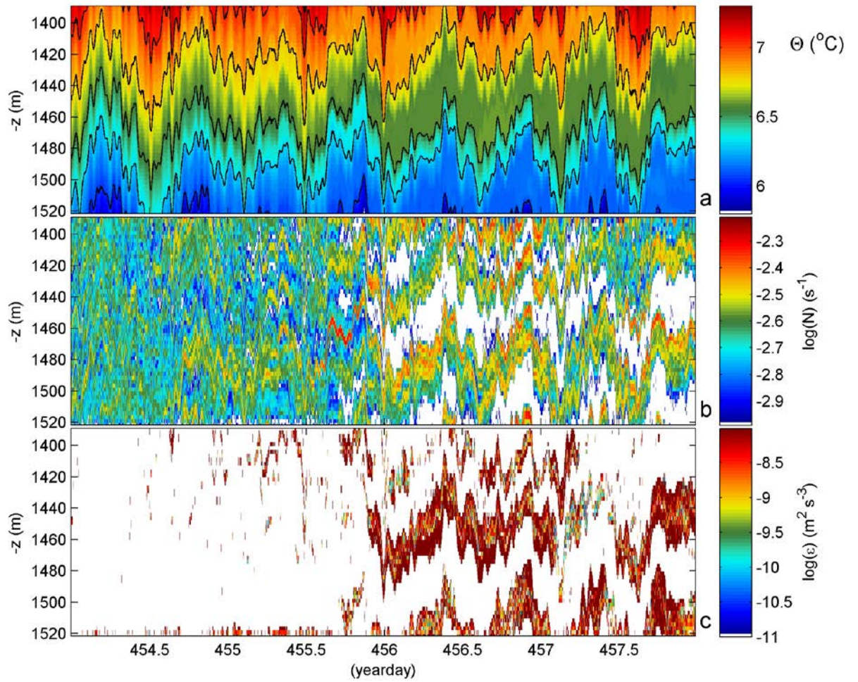
Figure 7. Same as Fig. 5, but around day 456 of the Meddy departing. Note the different temperature range in a.
