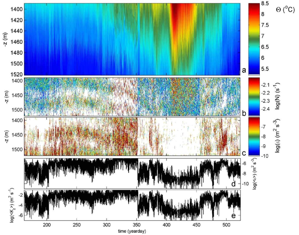
Figure 4. Same one year period as in Fig. 2, here providing an overview of T-sensor data. The passage of a Meddy above is noticeable in the discontinuities around days 352.5 and 456. (a) Conservative ( \sim potential) Temperature, with data from four sensors interpolated. (b) Logarithm of buoyancy frequency from the reordered version of a. (c) Logarithm of dissipation rate estimates from data in a., b. (see text). (d) Vertically averaged data of c. (e) Logarithm of vertically averaged eddy diffusivity.
