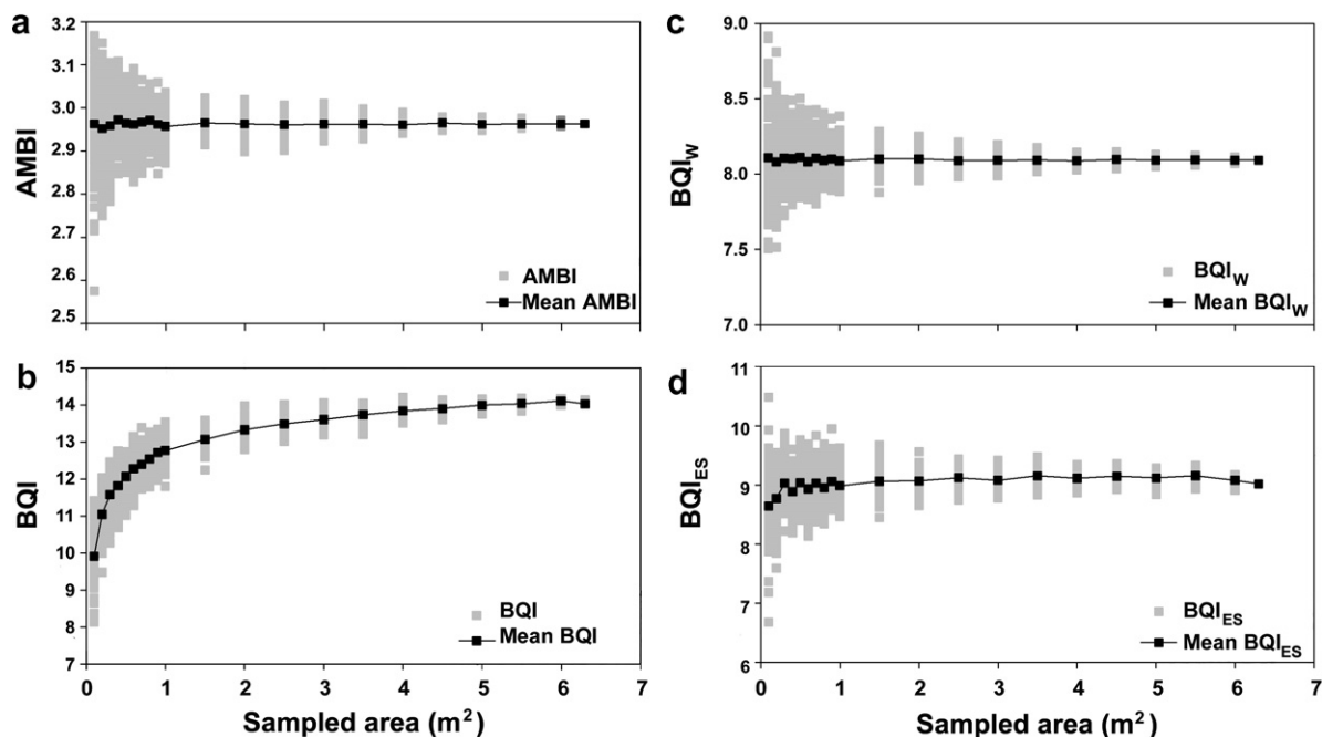
Fig. 2. The 63 independent replicates from the station ‘Millionenviertel 14’ in the western Baltic Sea (Fig. 1‘A’) were used for 1964 permutations to simulate increasing sampling effort. The sampling effort plotted against the four different quality indices AMBI (a), BQI (b), BQI_W (c) and BQI_{ES} (d).
