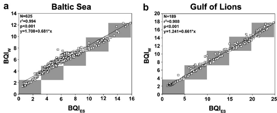
Fig. 5. Showing the large data sets from the Southern Baltic and Gulf of Lions. The EcoQ classification relationship between BQI W and BQI ES . Shaded areas indicate that similar EcoQs are derived from the two considered indices.
