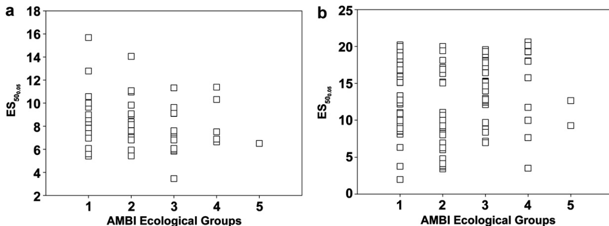
Fig. 7. Showing the relationship between the two different ways of species sensitivity/tolerance level classification (AMBI ecological groups and ES_{50,05} calculation) for the large data sets from Southern Baltic (a) and Gulf of Lions (b).
