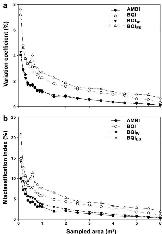
Fig. 3. Relationships between variation coefficients (a) and misclassification indices (b) of AMBI, BQI, BQI W , and BQI ES versus sampling effort at 'Millionenviertel 14' from the western Baltic Sea.
