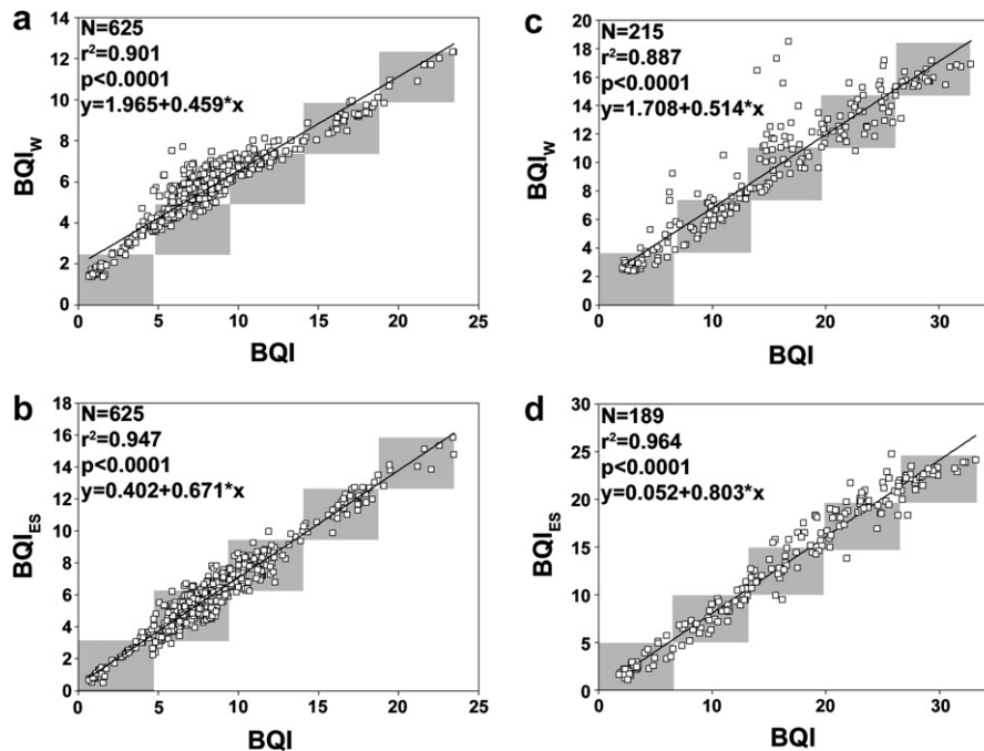
Fig. 4. Showing the large data sets from Southern Baltic (a and b) and Gulf of Lions (c and d). The EcoQ classification relationship between BQI and BQI W (a and c), and BQI ES (b and d). Shaded areas indicate that similar EcoQs are derived from the two considered indices.
