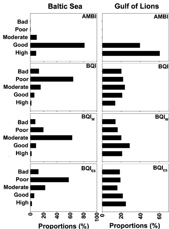
Fig. 6. Showing the large data sets from Southern Baltic Sea and Gulf of Lions and the frequency distribution of EcoQ based on AMBI, BQI, BQI w , and BQI ES in these two far apart areas.
