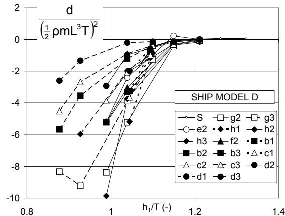
Figure 6.10: Discriminant of quadratic equation for stability indices: influence of bottom characteristics and under keel clearance.
