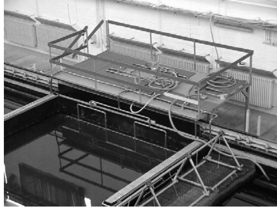
Figure 4.5. Flanders Hydraulics Research shallow water tank: mud reservoir with pump system.
