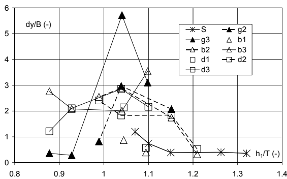
Figure 7.26. Course change of 30 deg to starboard at harbour full ahead, R = 1500 m – model D – maximal lateral deviation. Influence of bottom characteristics and under keel clearance.
