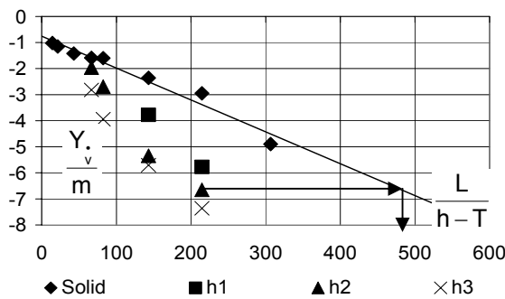
Figure 10.8. Sway added mass, ship model D, u > 0 , 0 rpm. Illustration of the effect of the fluidization parameter.
